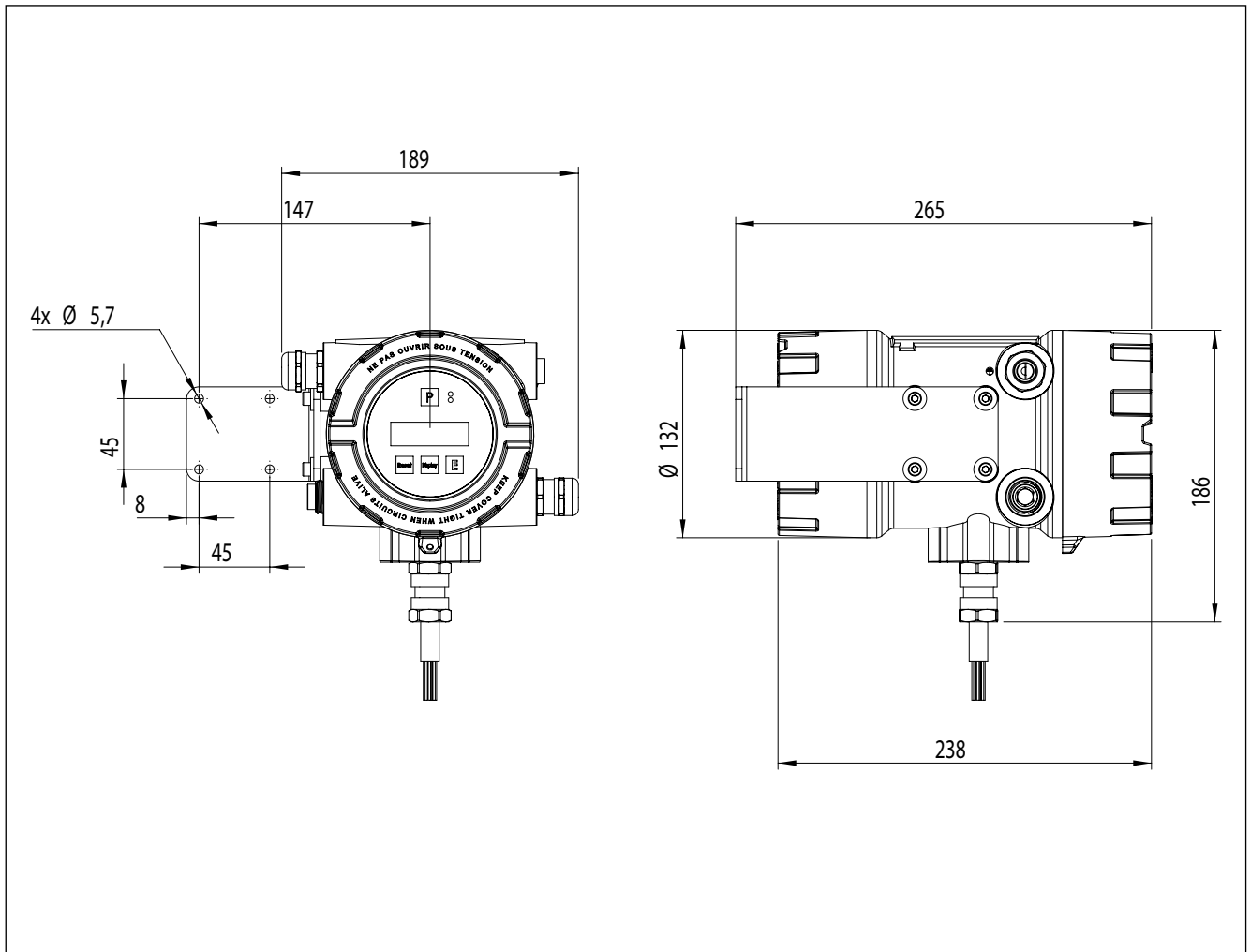
Dimensional drawing (mm) KCE 80xx - WE with cable connection
