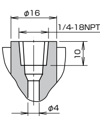
DETAIL "B" (PRESS. CONN.) 4th digit code "6,7,8,9"
