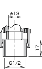
DETAIL "C"
