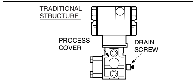
Figure 3. Vertical Mounting - Cavity Draining
