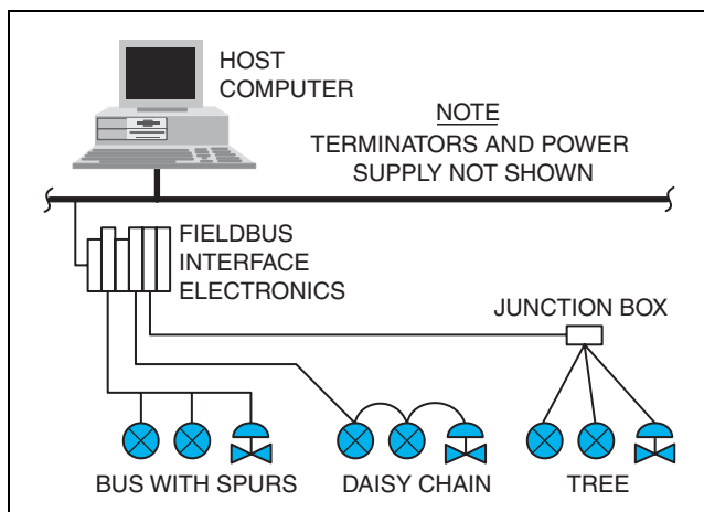
Figure 20. Fieldbus Miscellaneous Topologies
