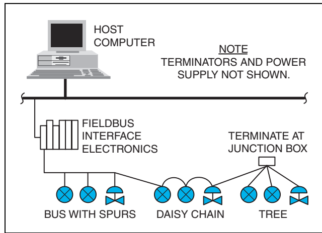
Figure 23. Fieldbus with Mixed Topologies
